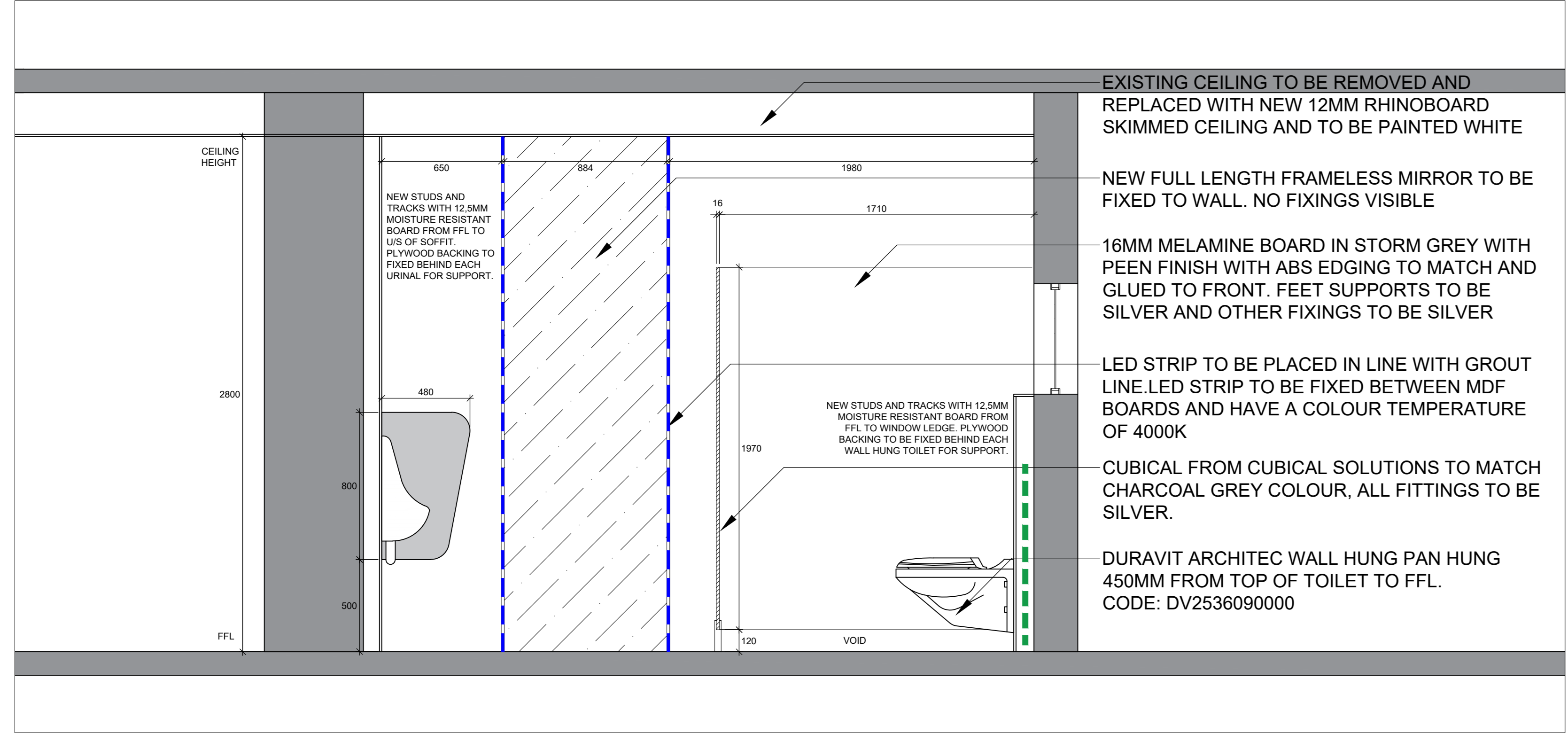
C. ELEVATION B-B SCALE 1:20
