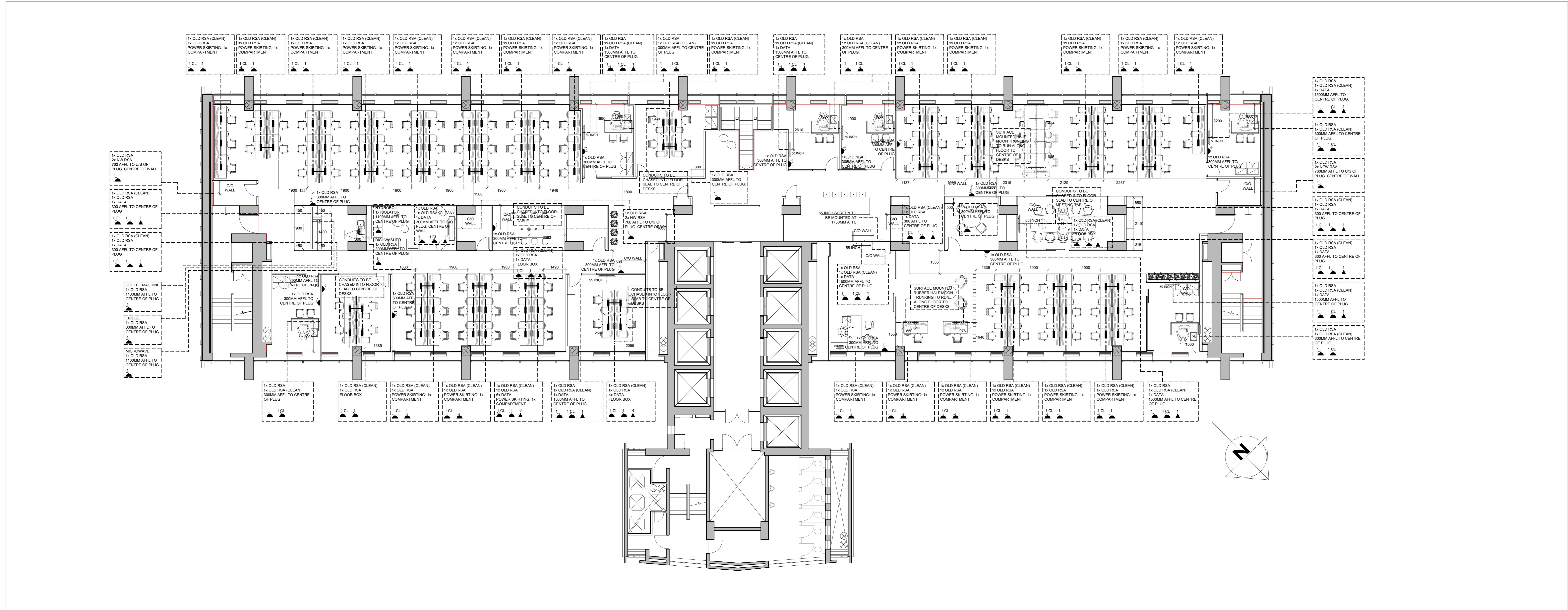
8TH FLOOR PLAN SCALE: 1:100
