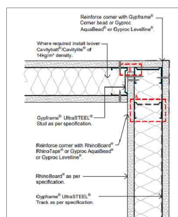
04. DETAIL 04 - PARTITION CORNER DETAIL SCALE 1:5
