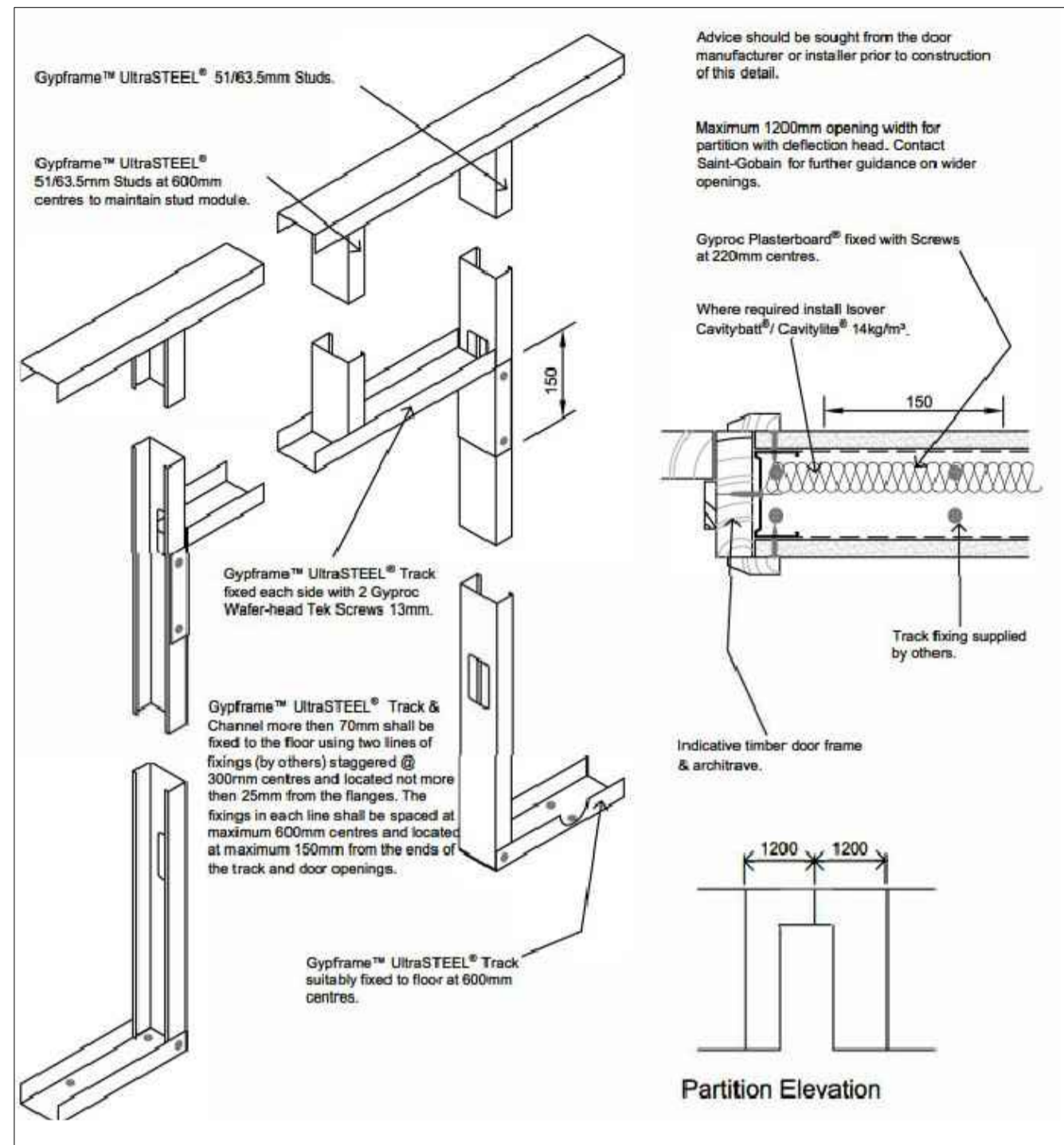
12. DETAIL 12 - DOOR OPENING SCALE 1:5
