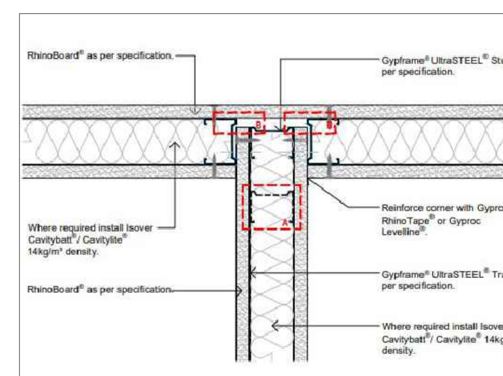
06. DETAIL 06 - PARTITION T-JUNCTION DETAIL SCALE 1:5
