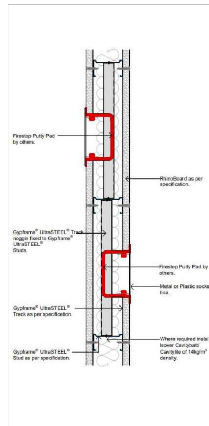
09. DETAIL 09 - SOCKET WITH ULTRASTEEL FRAMEWORK & PUTTY PAD 60MIN FIRE RATING SCALE 1:5
