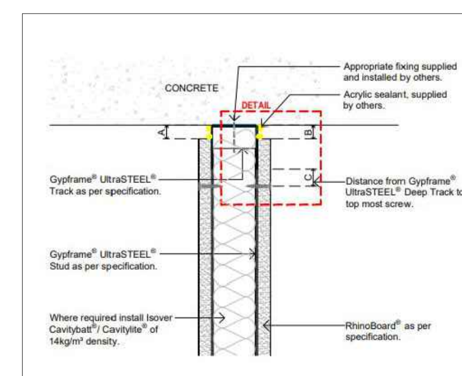
05. DETAIL 05 - PARTITION SOFFIT DETAIL SCALE 1:5
