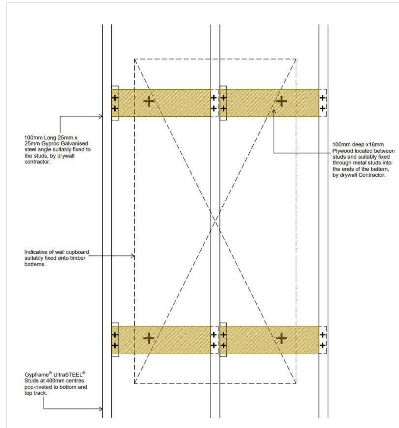
13. DETAIL 13 - CUPBOARD FIXING SCALE 1:5
