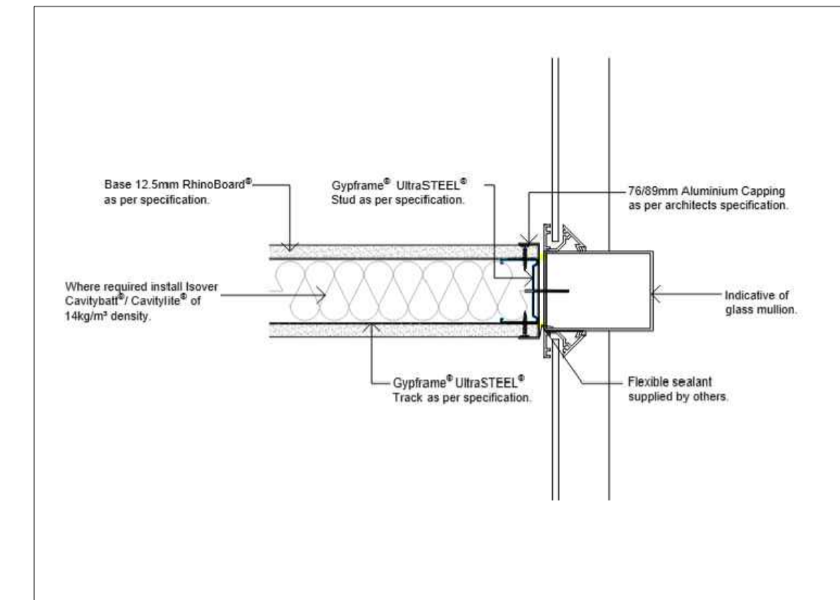
15. DETAIL 15 - ABUTMENT DETAIL - PARTITION TO MULLION SCALE 1:5
