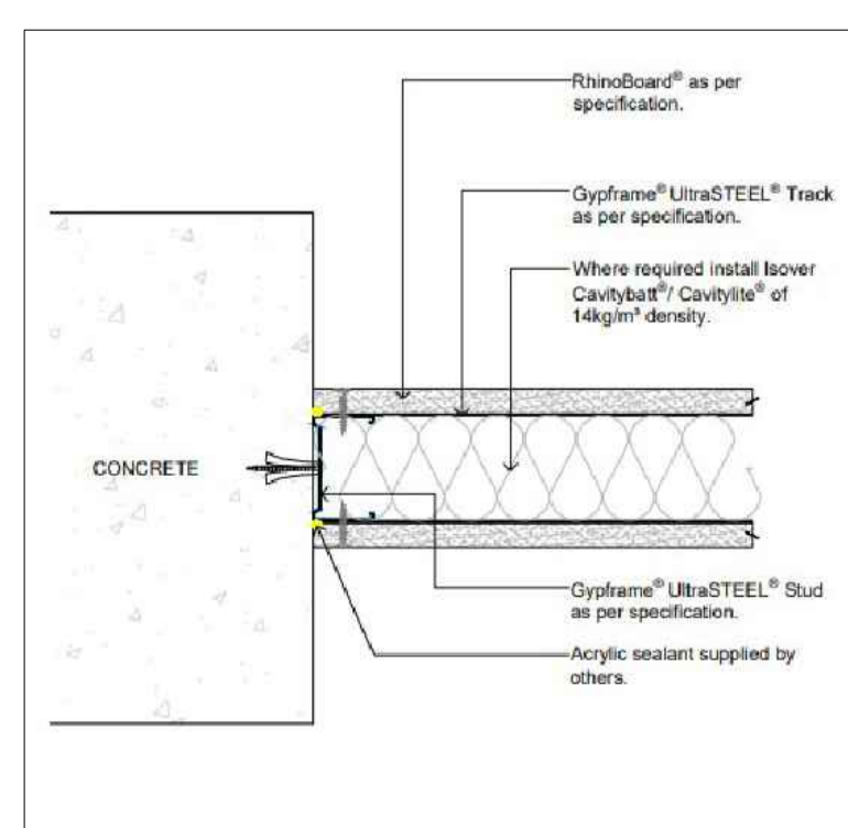
02. DETAIL 02 - ABUTMENT DETAIL - COLUMN & PARTITION SCALE 1:5
