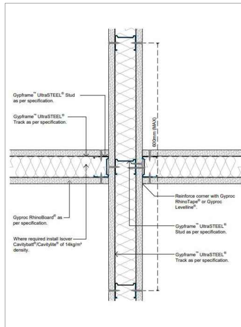
08. DETAIL 08 - PARTITION CROSS SECTION DETAIL SCALE 1:5
