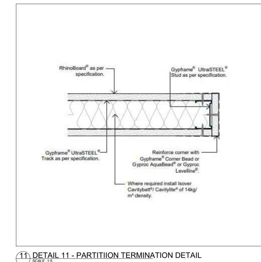
11. DETAIL 11 - PARTITION TERMINATION DETAIL SCALE 1:5
