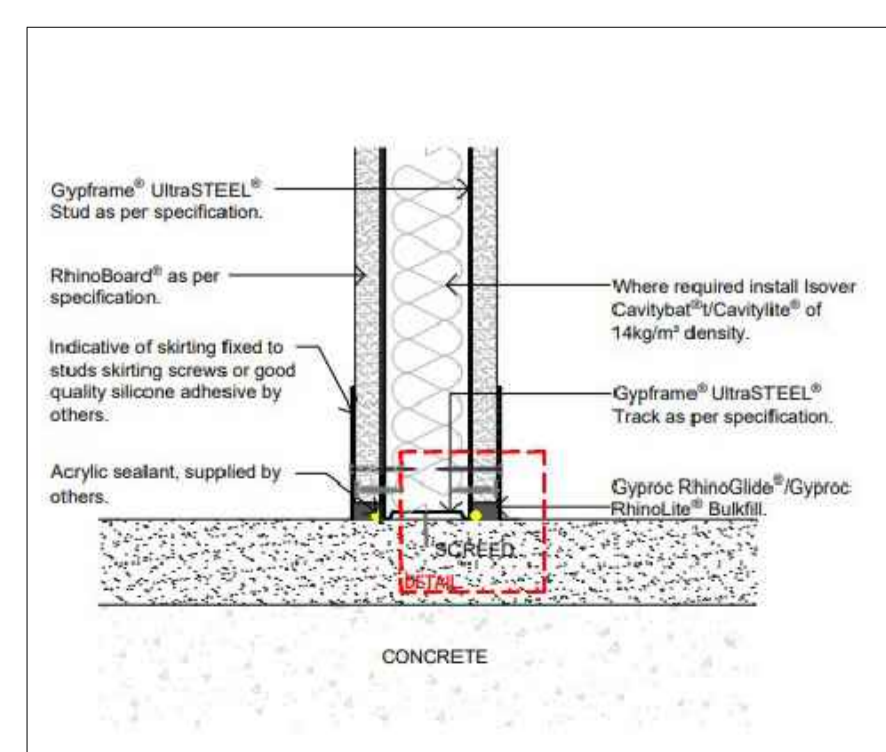
03. DETAIL 03 - BASE DETAIL - ALUMINIUM SKIRTING SCALE 1:5
