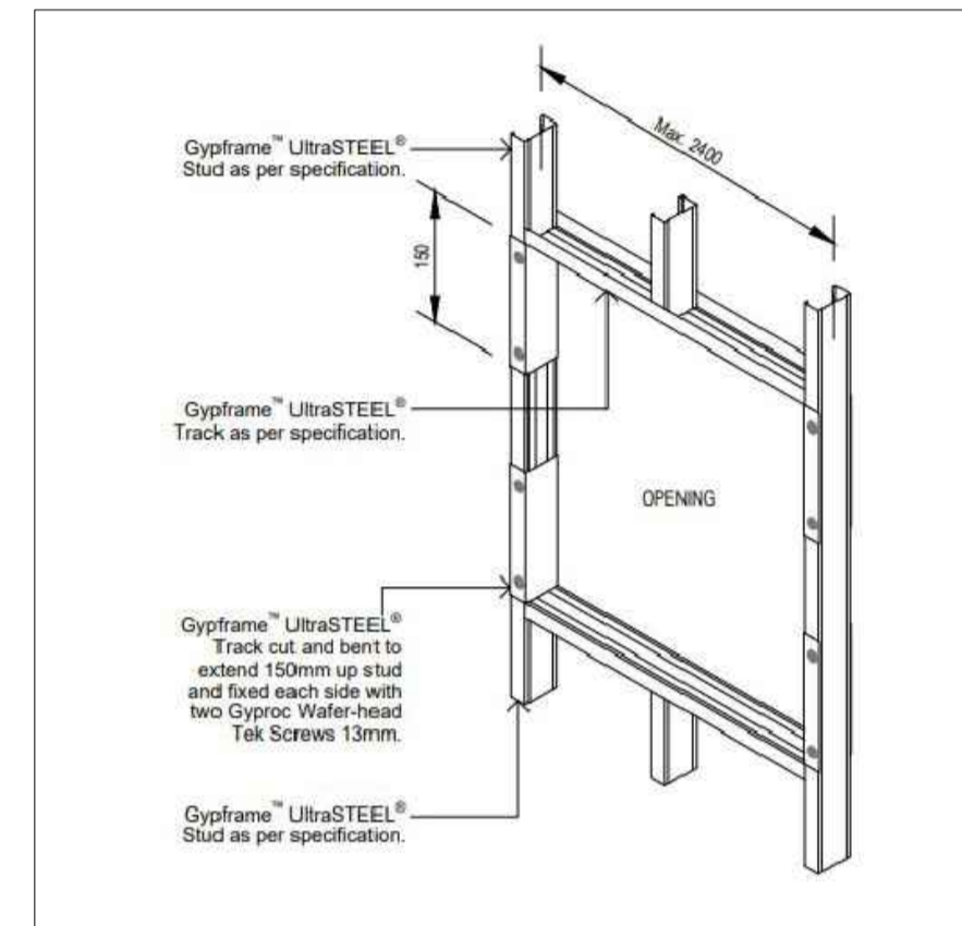
14. DETAIL 14 - FRAMEWORK PENETRATIONS SCALE 1:5
