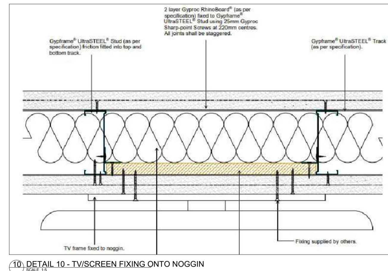
10. DETAIL 10 - TV/SCREEN FIXING ONTO NOGGIN SCALE 1:5
