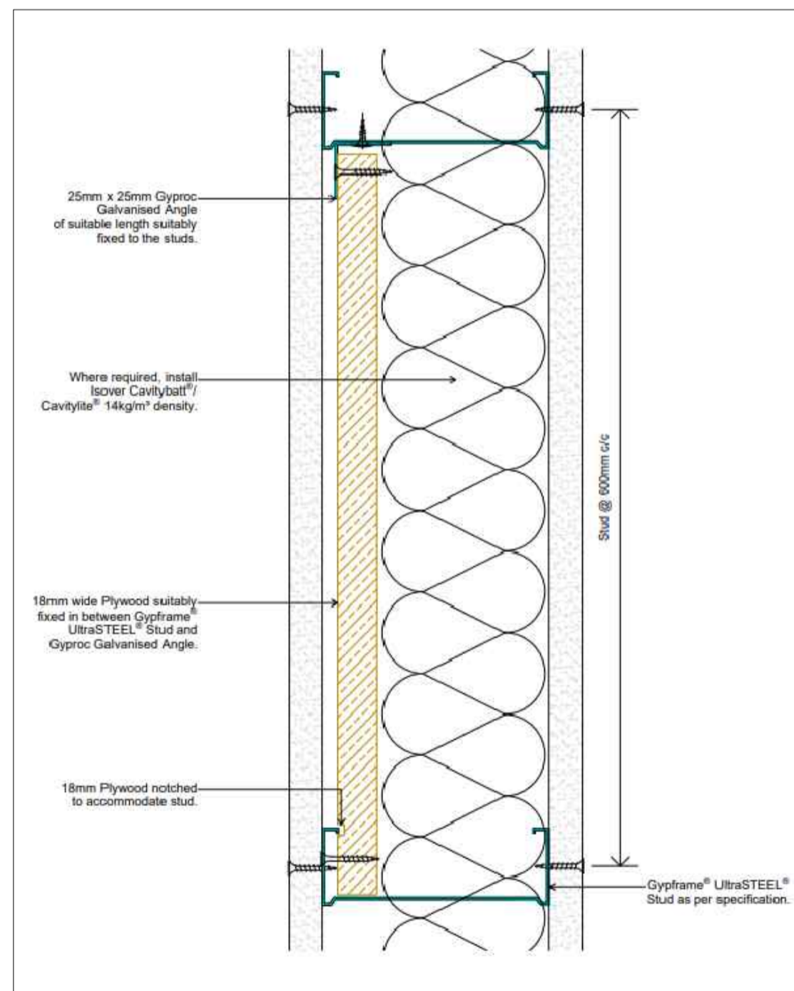
07. DETAIL 07 - PARTITION NOGGIN DETAIL SCALE 1:5
