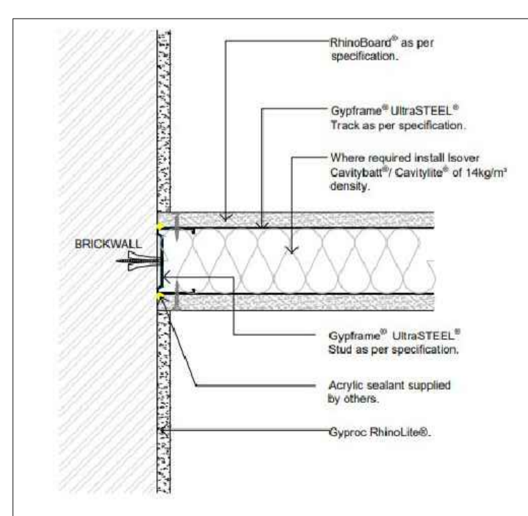
01. DETAIL 01 - ABUTMENT DETAIL - WALL & PARTITION SCALE 1:5
