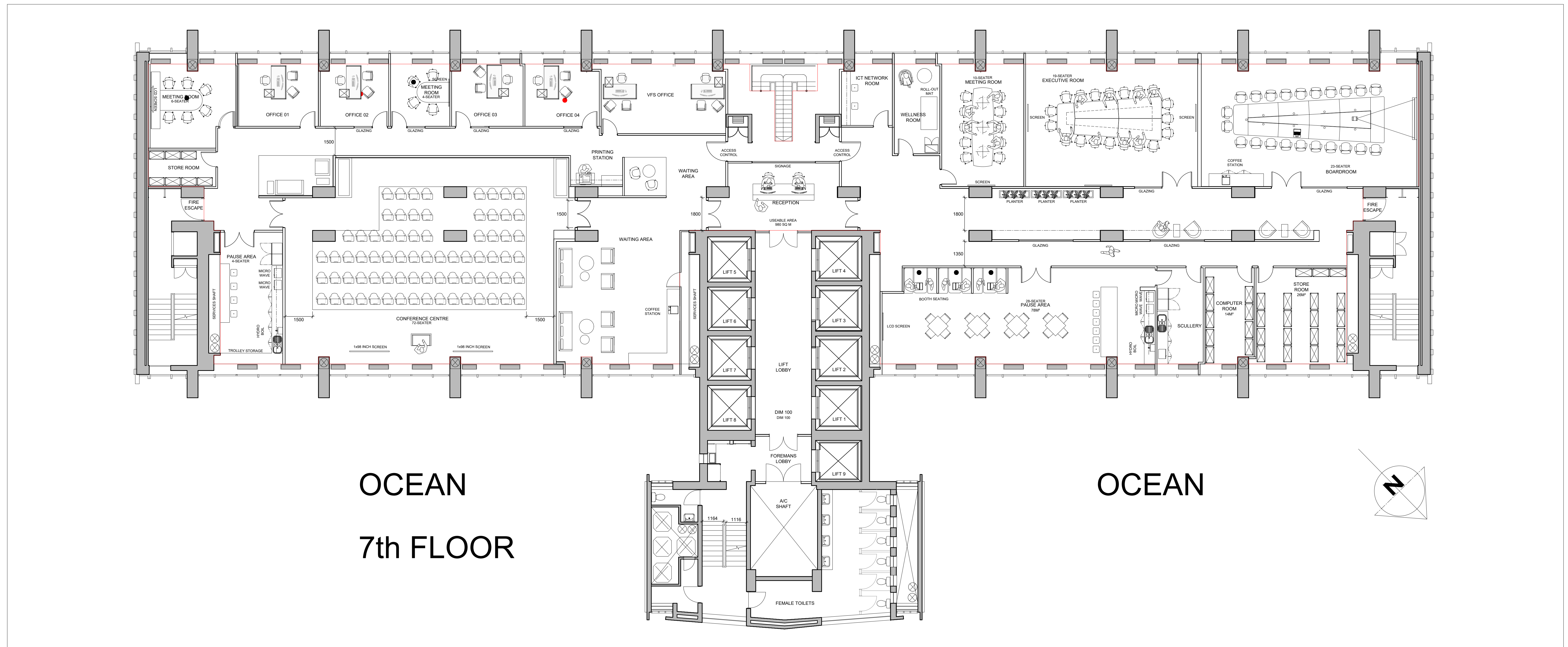
01: 7TH FLOOR PLAN SCALE: 1:100
